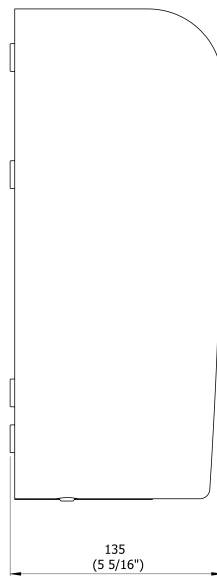
GW01 40 04 01 AISI304 Stainless steel brushed
