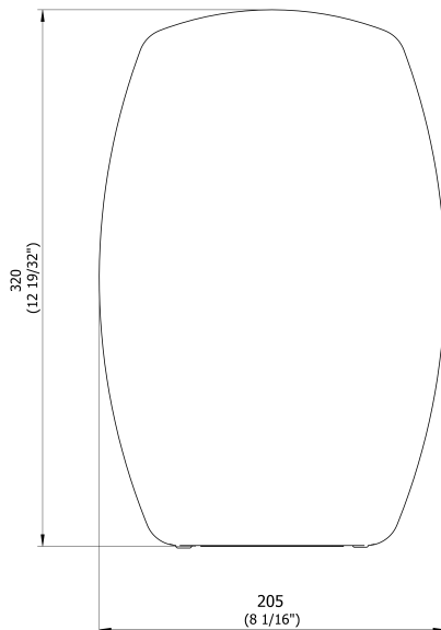
GW01 40 04 00 AISI304 Stainless steel white
